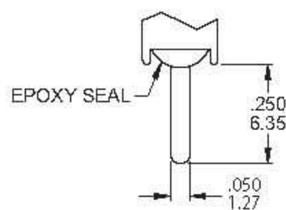
M2 PC Thru-hole
